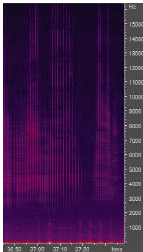
Figure 35 : clics de cachalot
